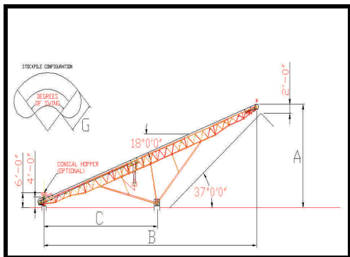
FIXED ELEVATION RADIAL STACKER MODEL 636
